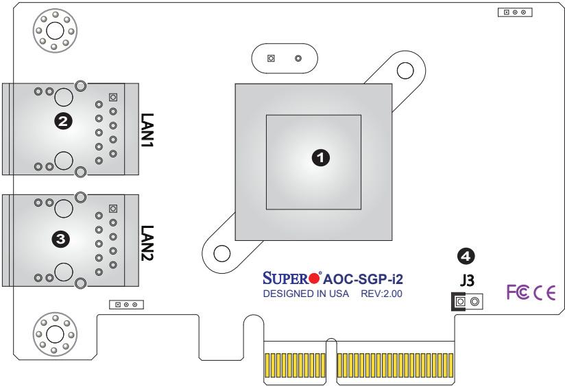
AOC-SGP-i2 Layout
