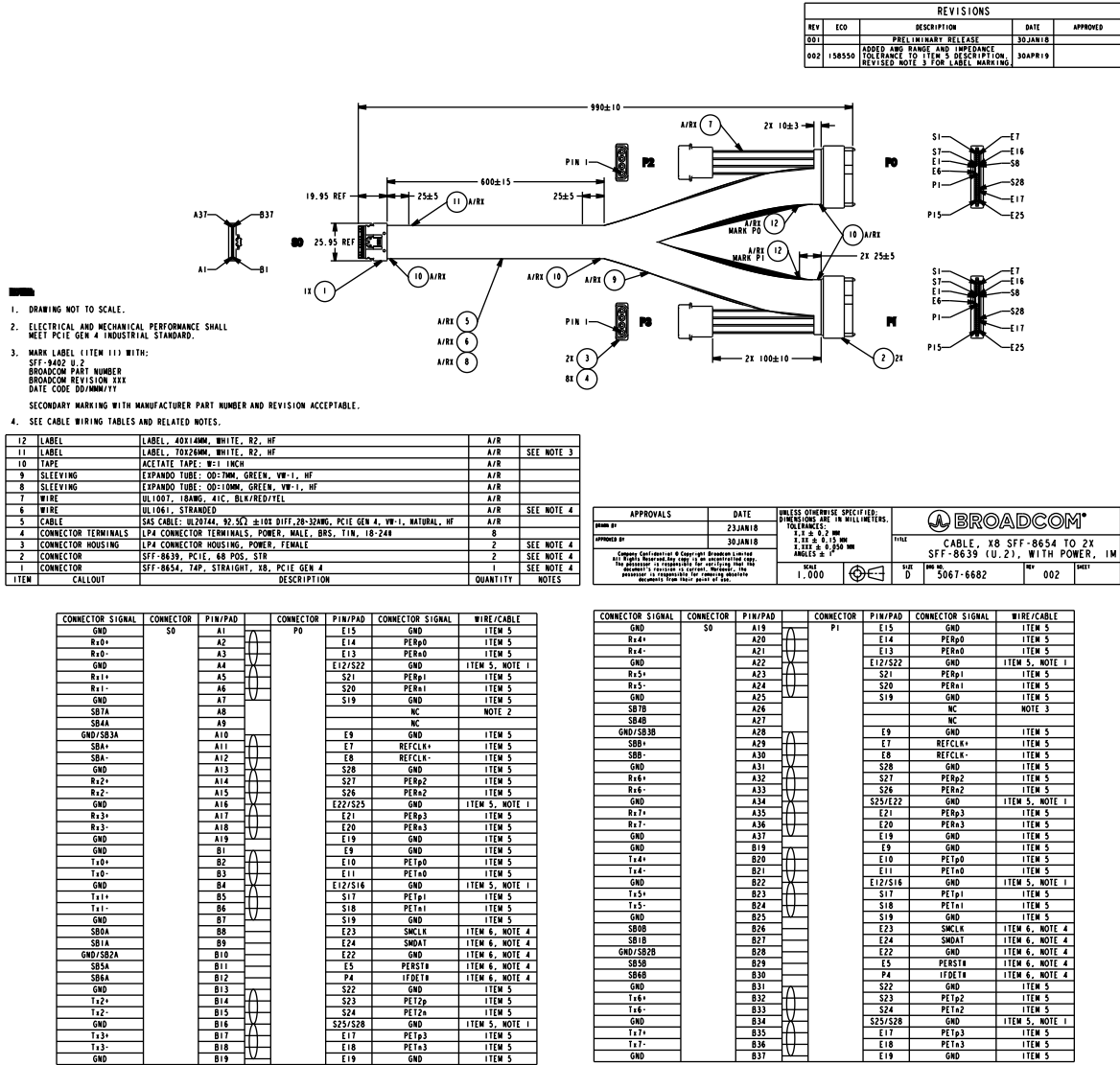
Figure 19: Cable 05-60005-00 Drawing and Pinout
